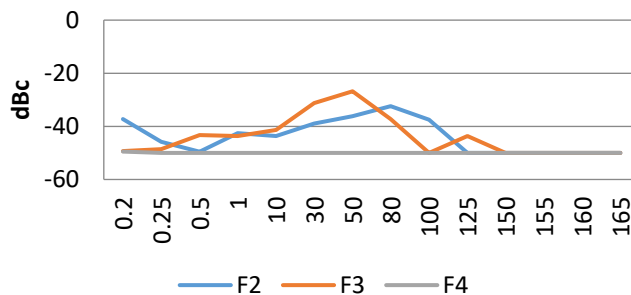
Harmonics at 100 W
