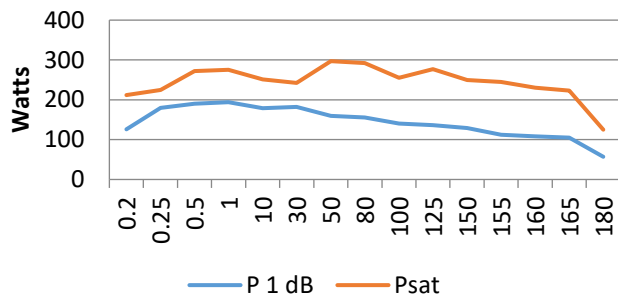
Power v Frequency
