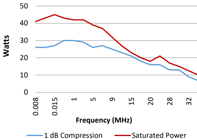
210L Extended Power Data
