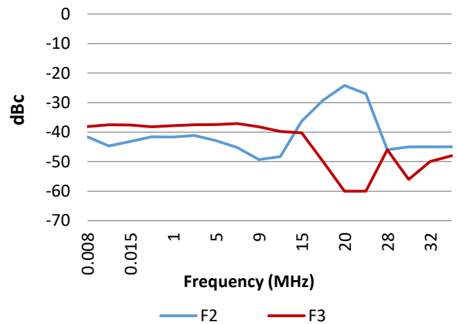
Harmonics @10W P OUT
